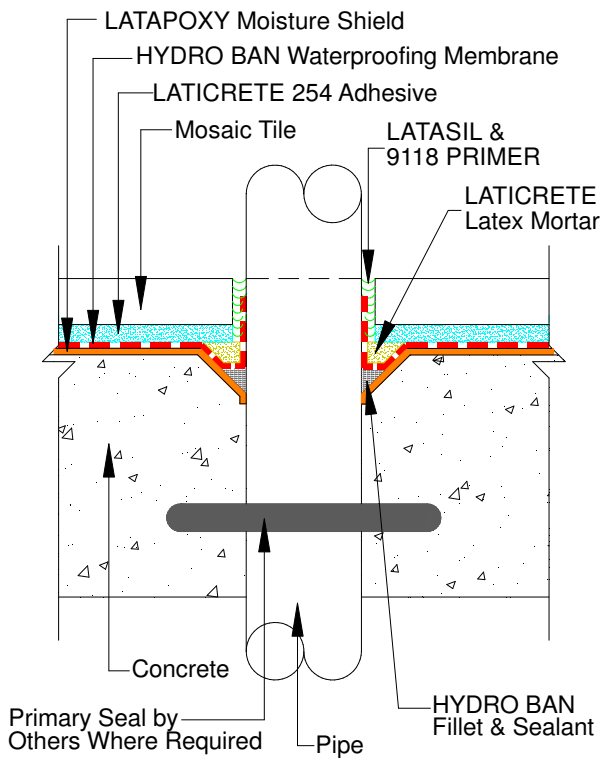
Detail 5 - Immersed Installation Pipe Penetration
