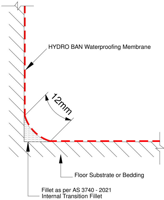
Detail 1 - Bond Relief Fillet
