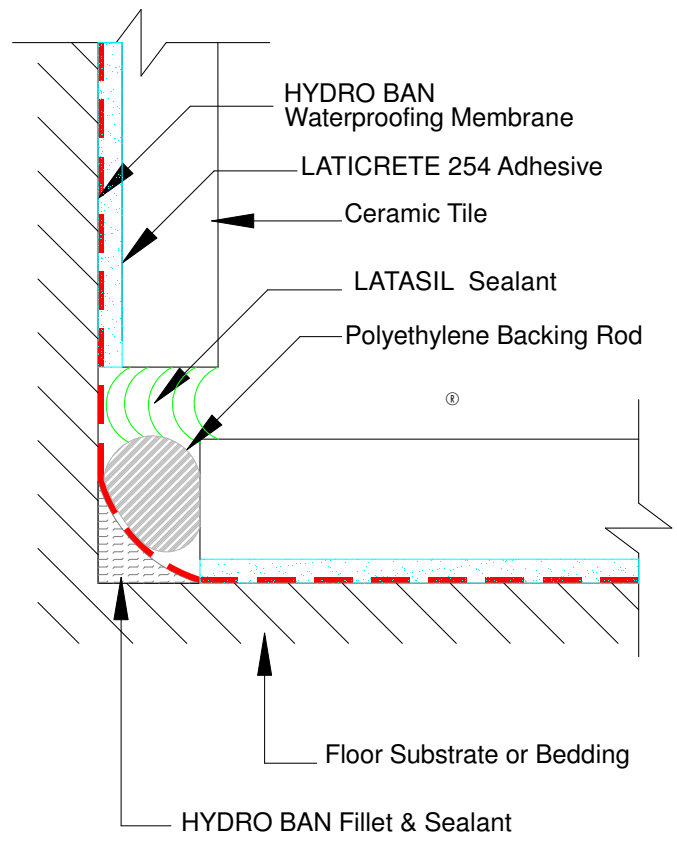
Detail 2 - Typical Thin Bed Installation
