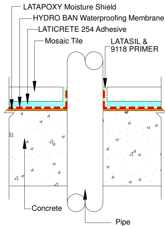
Detail 6 - Pipe Penetration
