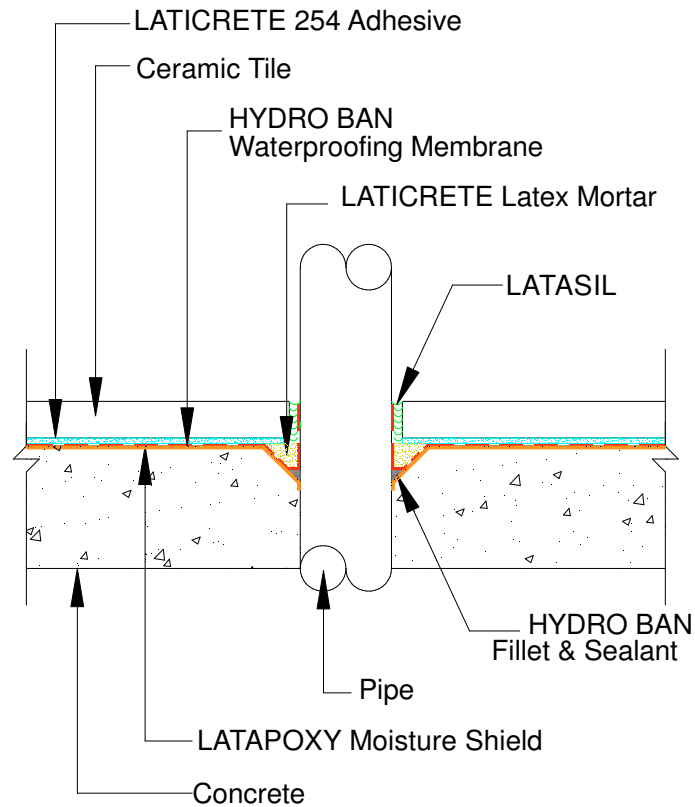
DETAIL 2 Immersed Pipe Penetration
