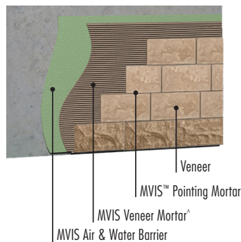
Masonry Veneer Installation System
