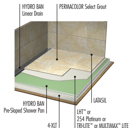
HYDRO BAN® Shower System Linear Drain
