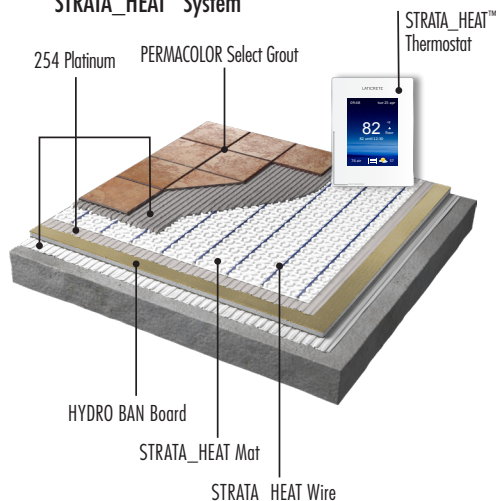
STRATA_HEAT™ System
