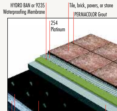
Tile Drain Mat 3701 Fortified Mortar with wire-reinforcing Primary roof waterproofing membrane Structural concrete deck, properly pitched
