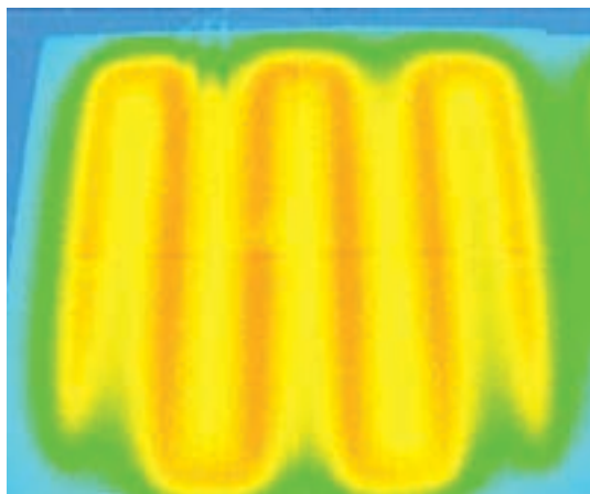
Infrared image using STRATA_HEAT™ Thermal Pack 1 diffuses heat uniformly throughout — no cold spots
