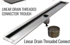
Linear Drain Threaded Connector designed to connect to clamping ring drain assemblies. Trough
